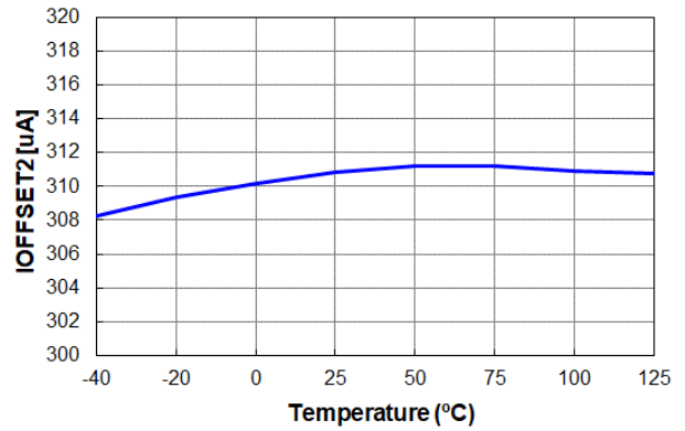
Figure 4. I OFFSET2 vs. Temperature
