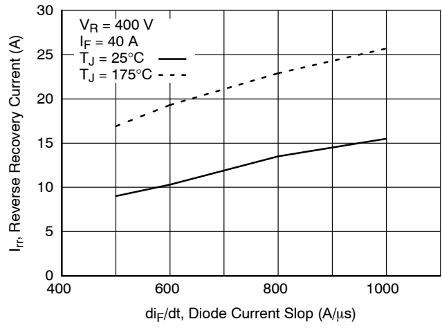
Figure 16. Reverse Recovery Current
