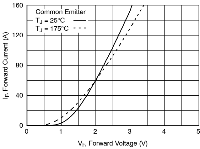
Figure 15. Forward Characteristics
