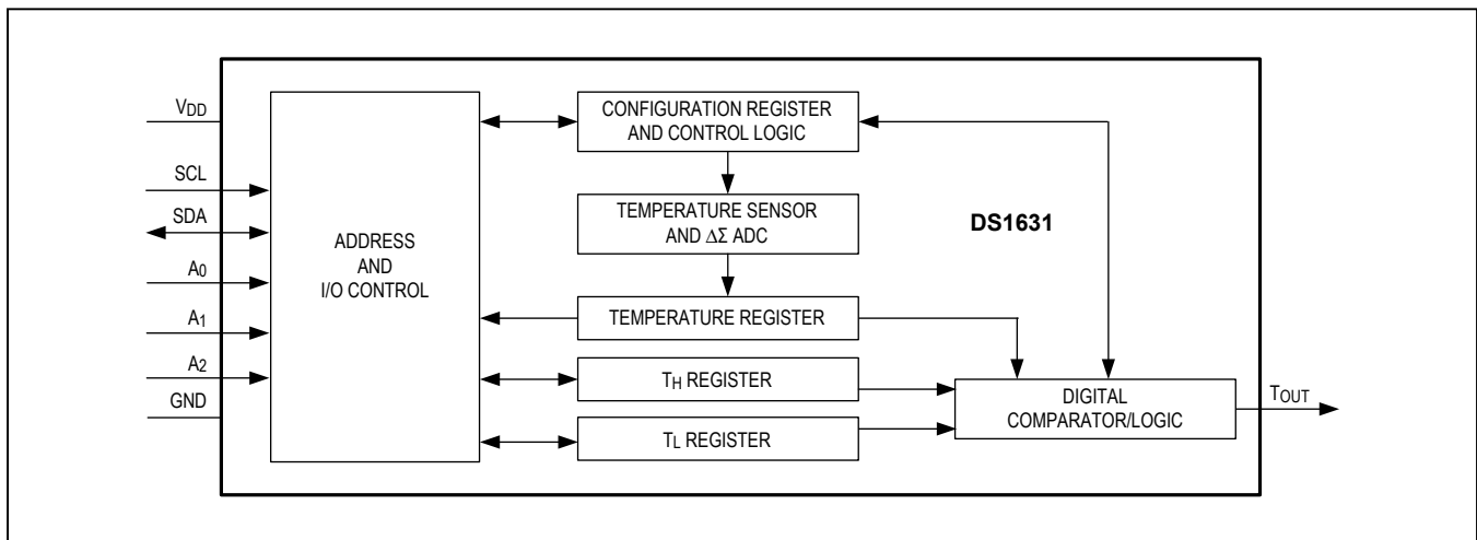
Figure 1. Functional Diagram
