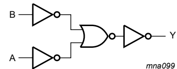
Fig. 3. Logic diagram
