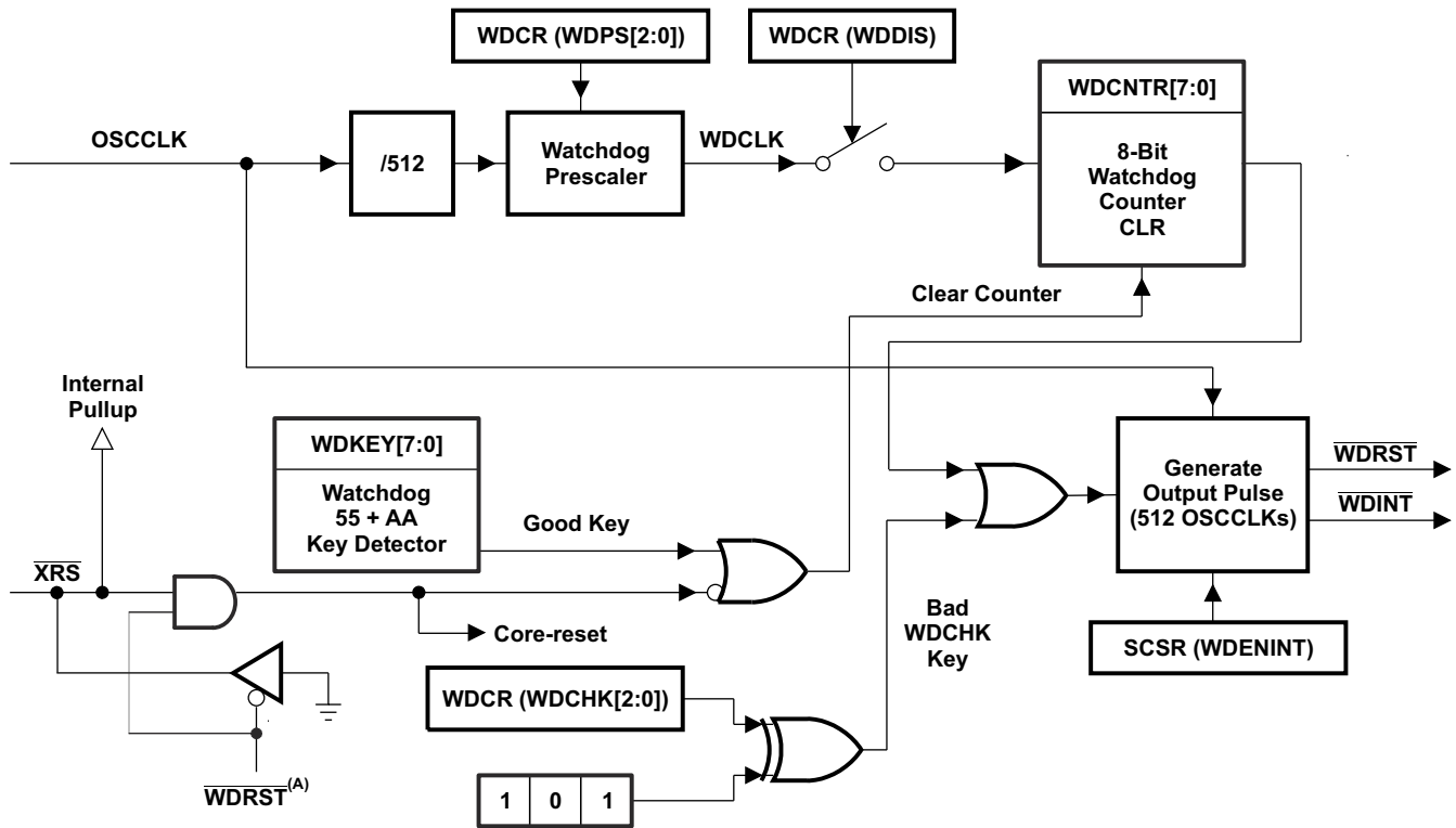
Figure 9-30. Watchdog Module
