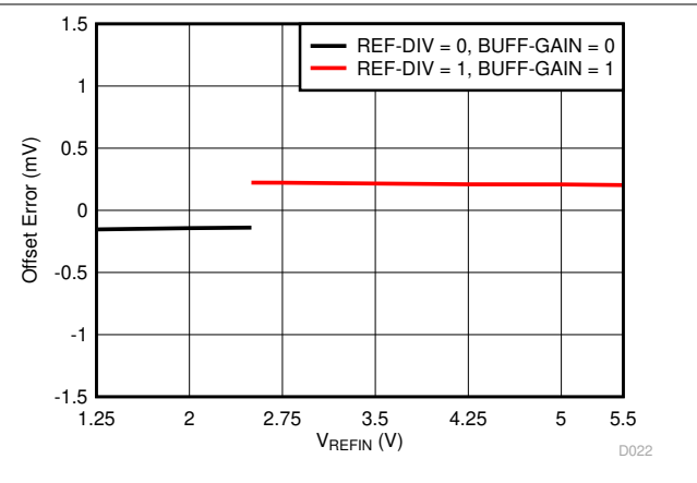
Figure 7-24. Offset Error vs Reference Voltage
