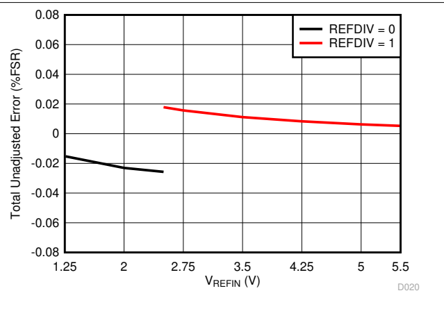
Figure 7-22. Total Unadjusted Error vs Reference Voltage
