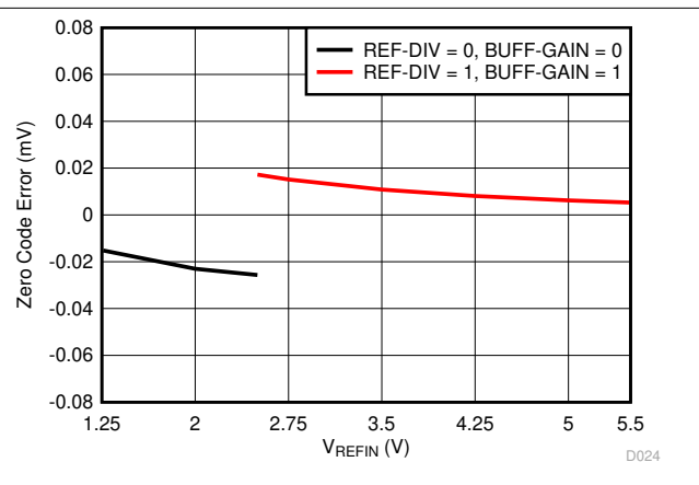
Figure 7-26. Full Scale Error vs Reference Voltage
