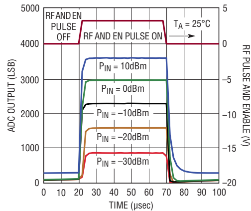
Output Transient Response with RF Pulse and EN Pulse
