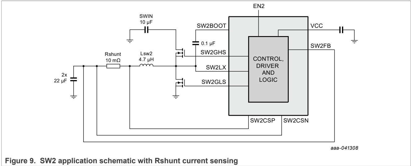
Figure 9. SW2 application schematic with Rshunt current sensing
