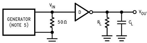
Figure 2. Driver Propagation Delay and Slew Rate Test Circuit
