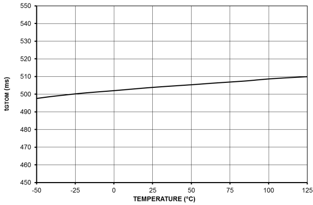
Figure 34. Go To Off Mode Timer Duration t GTOM
