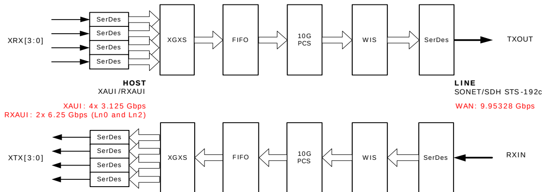
Figure 74 • 10G WAN
