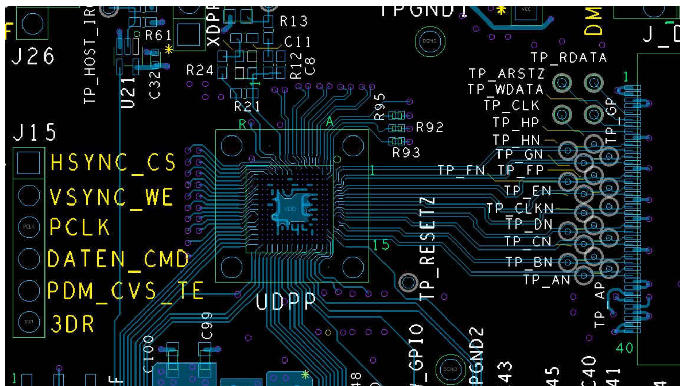
Figure 10-3. Layout Recommendation
