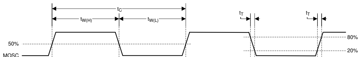
Figure 6-5. System Oscillators
