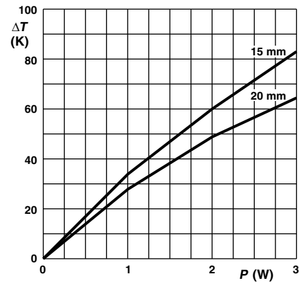
\varnothing 0.78 mm Cu-leads Minimum distance from resistor body to PCB = 1 mm
