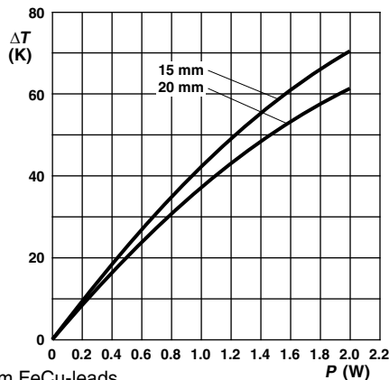
\varnothing 0.78 mm FeCu-leads Minimum distance from resistor body to PCB = 1 mm
