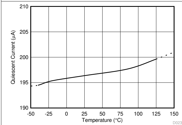
Figure 7-23. Quiescent Current vs. Temperature (INA180-Q1)
