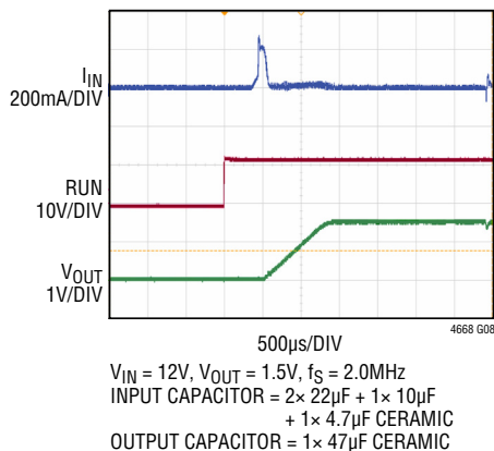
Start-Up with No Load
