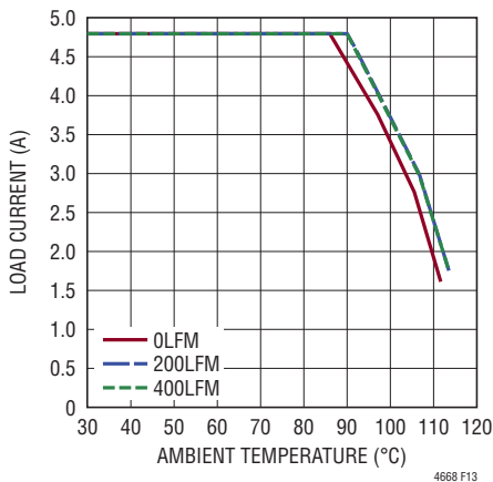
Figure 13. 12V to 0.8V Derating Curve, No Heat Sinking
