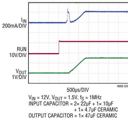
Start-Up with 1.5A Load
