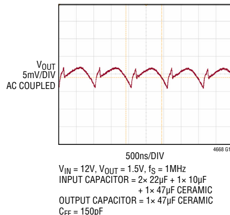
Output Ripple
