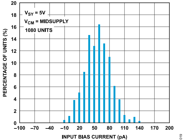
Figure 21. Typical Distribution of Input Bias Current, V_{SY} = 5\text{ V}
