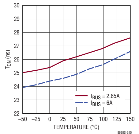
Top FET Minimum On-Time
