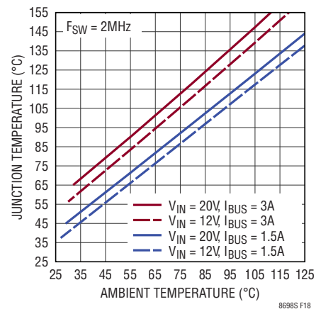
Figure 18. Junction Temperature Rise (DC2688A Demo Board with R_{SEN} = 8m\Omega )
