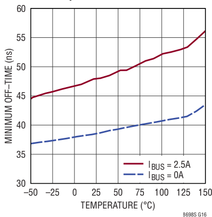
Minimum Off-Time vs Temperature
