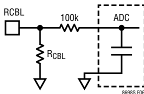
Figure 6. Using the RCBL Pin as Output Current Monitor
