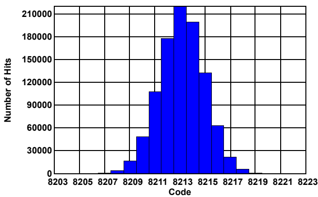
Figure 16. Noise Histogram
