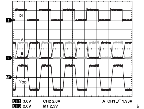
Figure 25. Driver Propagation Delay (Oscilloscope Plot), Data Rate = 500 kbps, 500 kbps Models
