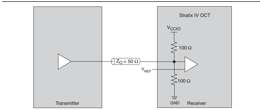
Figure 6-20. On-Chip Parallel Termination with Calibration
