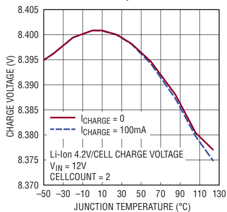
Charge Voltage (CV Mode) vs Junction Temperature
