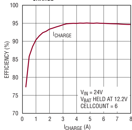
Lead-Acid Charging Efficiency vs I_{CHARGE}
