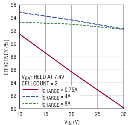
Li-Ion Charging Efficiency vs V_{IN}
