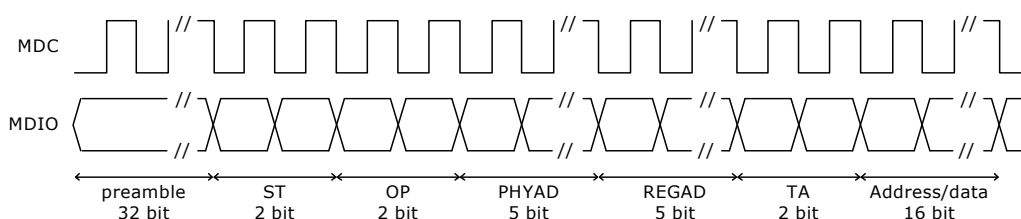
Figure 113 • MII Management Timing
