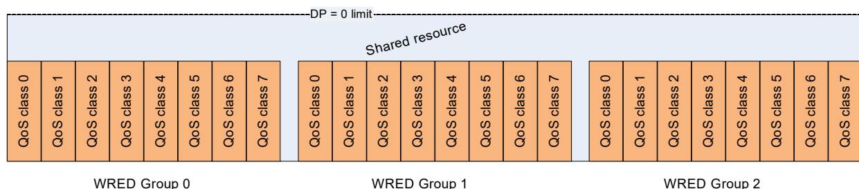
Figure 51 • WRED Sharing
