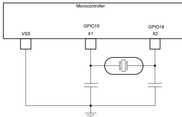
Figure 6-16. External Crystal
