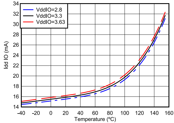
Figure 6-4. Current Versus Temperature – IDLE Mode
