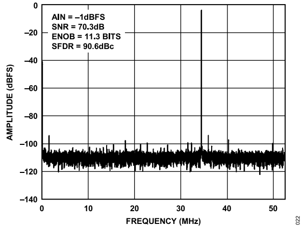
Figure 23. Single-Tone 16k FFT with f_{IN} = 140 \text{ MHz} , f_{SAMPLE} = 105 \text{ MSPS}
