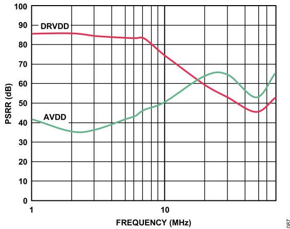
Figure 43. PSRR vs. Frequency, f_{CLK} = 125 MHz, f_{SAMPLE} = 125 MSPS
