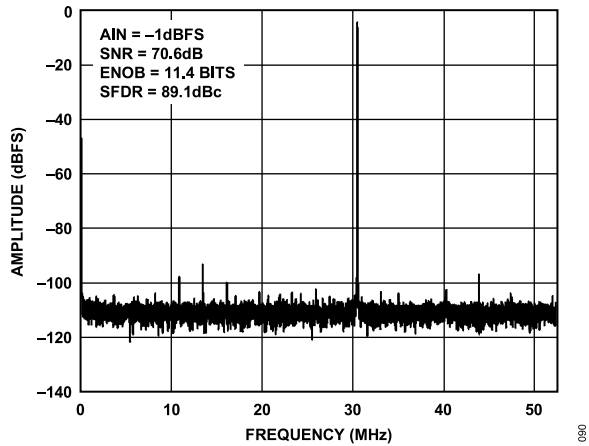
Figure 21. Single-Tone 16k FFT with f_{IN} = 30.5 \text{ MHz} , f_{SAMPLE} = 105 \text{ MSPS}
