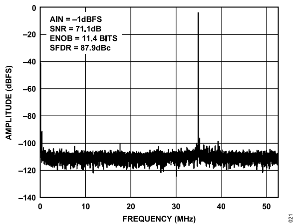
Figure 22. Single-Tone 16k FFT with f_{IN} = 70 \text{ MHz} , f_{SAMPLE} = 105 \text{ MSPS}
