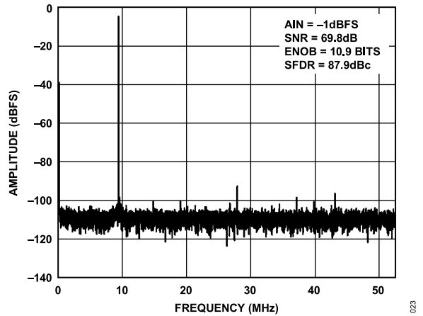
Figure 24. Single-Tone 16k FFT with f_{IN} = 200 \text{ MHz} , f_{SAMPLE} = 105 \text{ MSPS}
