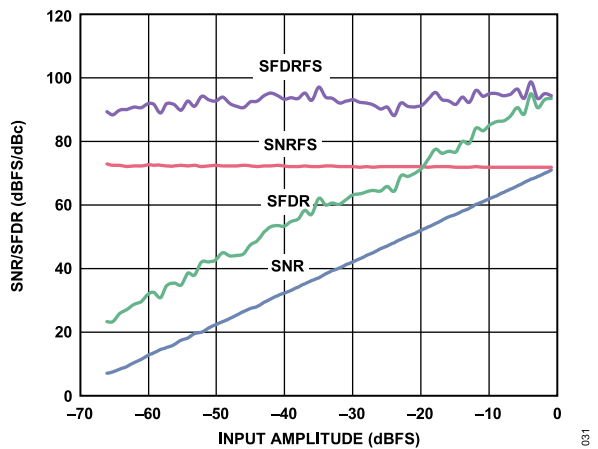
Figure 25. SNR/SFDR vs. Analog Input Level, f_{IN} = 9.7 \text{ MHz} , f_{SAMPLE} = 105 \text{ MSPS}
