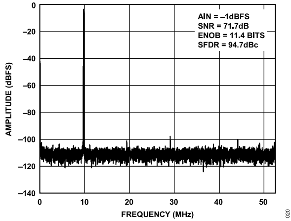
Figure 20. Single-Tone 16k FFT with f_{IN} = 9.7 \text{ MHz} , f_{SAMPLE} = 105 \text{ MSPS}
