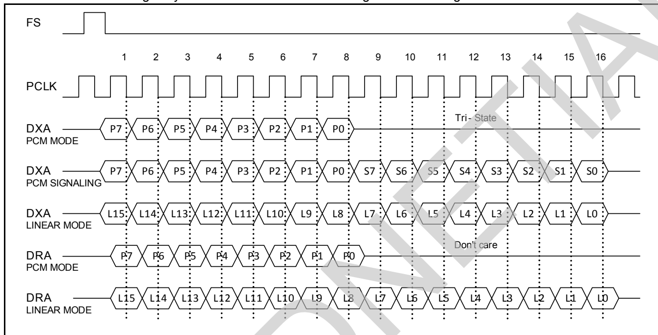
Figure 7 - PCM Data Flow Transmit and Receive Data (Transmit Data on Negative PCLK Edge)
