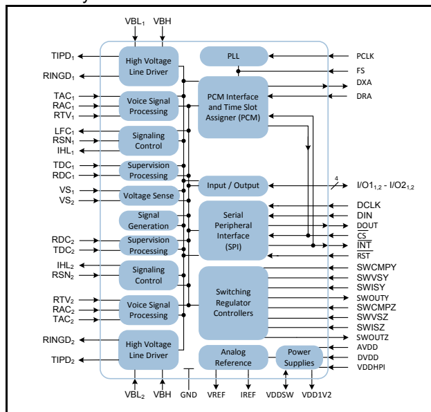
Figure 1 - Le9622 Device Block Diagram
