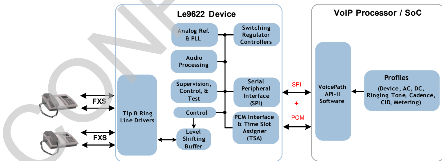
Figure 2 - Le9622 Dual-Channel VoicePort Solution Diagram
