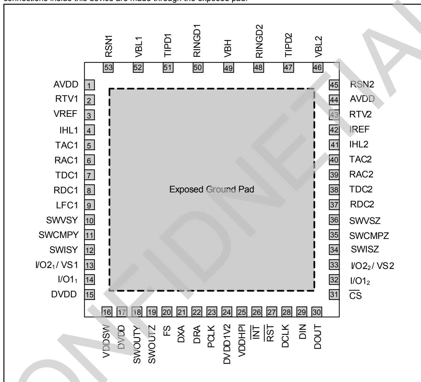
Figure 36 - Le9622 Device Pinout (QFN-53) - Top View
