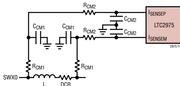
Figure 38. DCR Current Sensing Circuits
