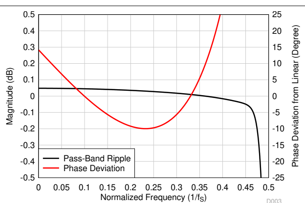
Figure 8-56. Ultra-Low-Latency Decimation Filter Pass-Band Ripple and Phase Deviation
