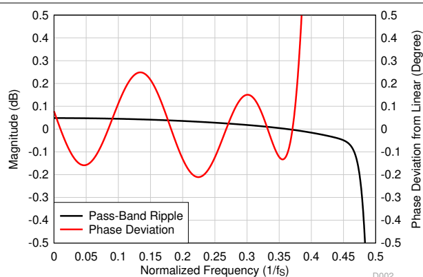
Figure 8-44. Low-Latency Decimation Filter Pass-Band Ripple and Phase Deviation
