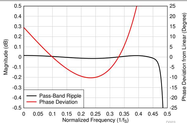
Figure 8-62. Ultra-Low-Latency Decimation Filter Pass-Band Ripple and Phase Deviation
