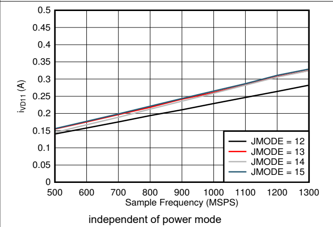
Figure 7-100. Dual Channel, I_{VD11} vs FS and JMODE 12 - 15
