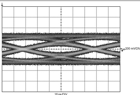
Figure 12. TL1 = 20 inch 4-mil FR4 Trace, TL2 = 15 inch 4-mil FR4 Trace, DS100KR800 Settings: EQ[1:0] = R, R = 15'h, DEM[1:0] = Float, Float
