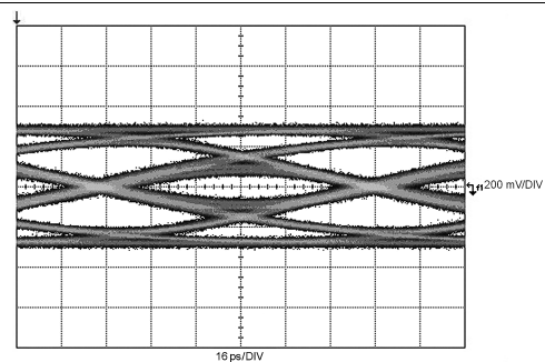
Figure 13. TL1 = 30 inch 4-mil FR4 Trace, TL2 = 15 Inch 4-mil FR4 Trace, DS100KR800 Settings: EQ[1:0] = Float, R = 1F'h, DEM[1:0] = Float, Float
