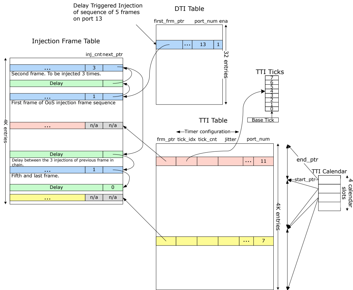
Figure 4-83. Injection Tables
