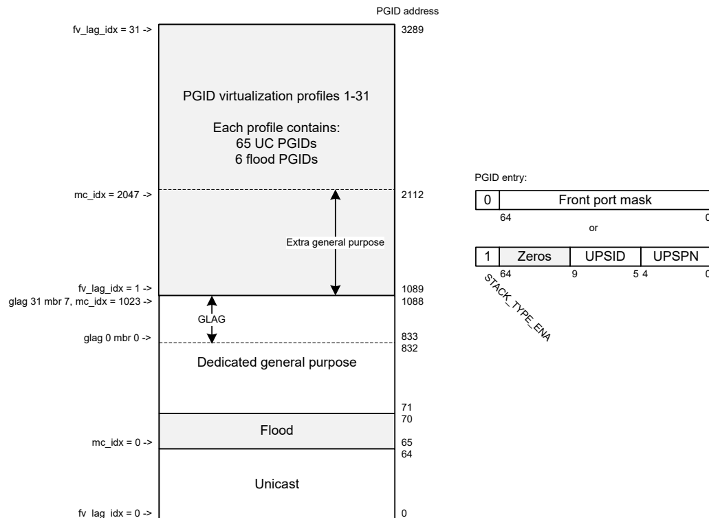
Figure 4-48. PGID Layout
