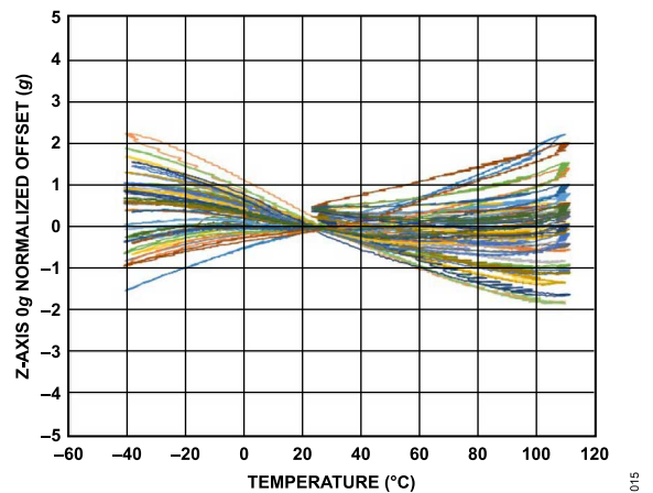
Figure 24. Z-Axis 0 g Normalized Offset vs. Temperature, 36 Devices Soldered to PCB, ODR = 2560 Hz
