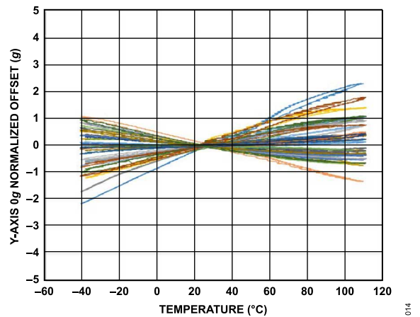
Figure 23. Y-Axis 0 g Normalized Offset vs. Temperature, 36 Devices Soldered to PCB, ODR = 2560 Hz
