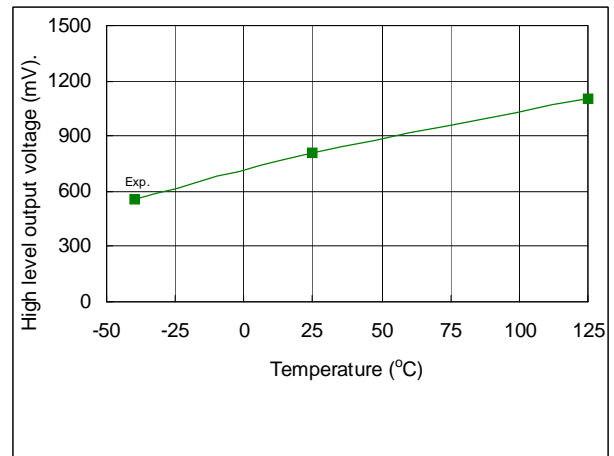
Figure 42. High Level Output Voltage vs. Temperature
