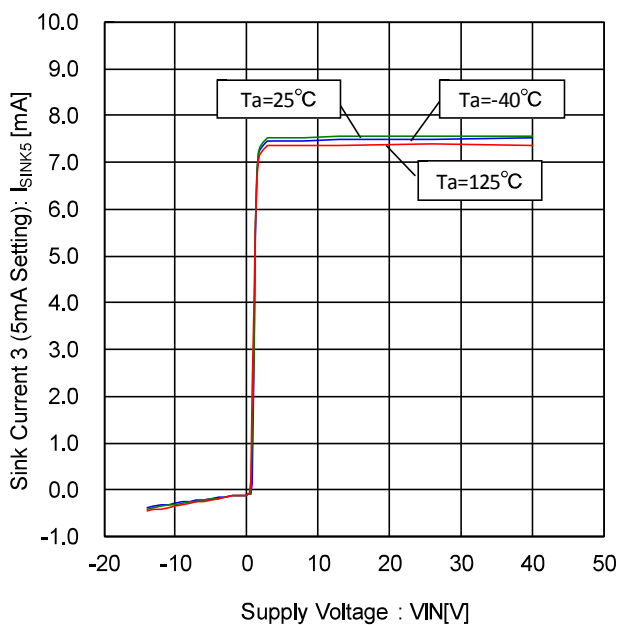
Figure 54. Sink Current 3- Voltage Characteristic (5mA Setting)
