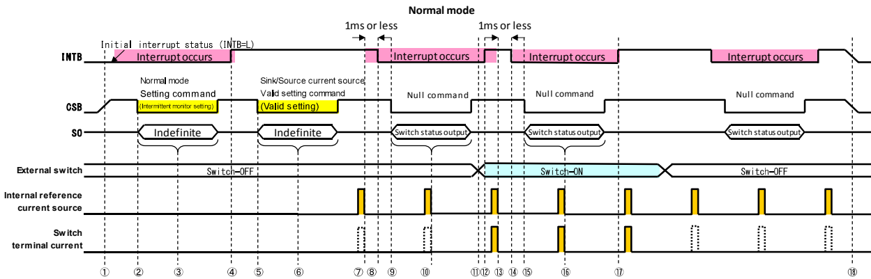
Figure 8. Basic Operation 2
