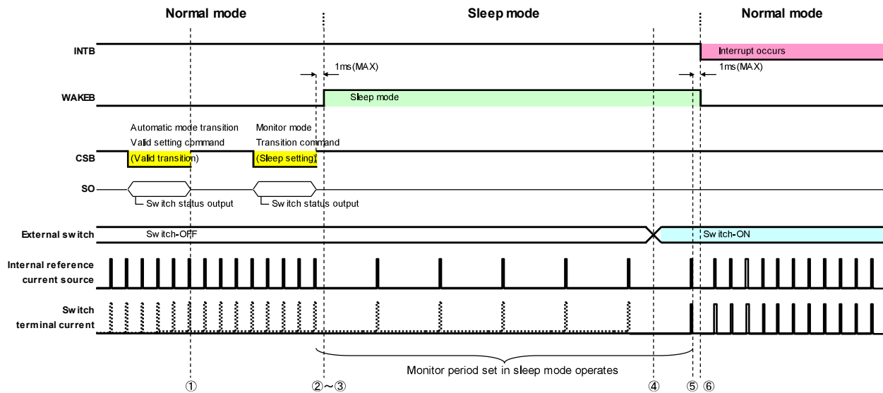
Figure 10. Basic Operation 4
