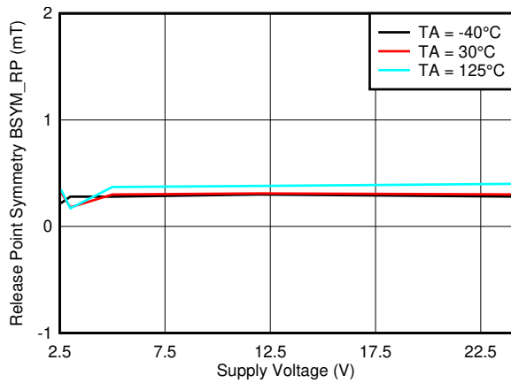
Figure 7-31. B_{SYM\_RP(ZY)} vs. V_{CC}
