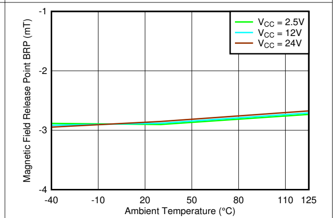
Figure 7-42. B_{RP\_Z} Threshold vs. Temperature
