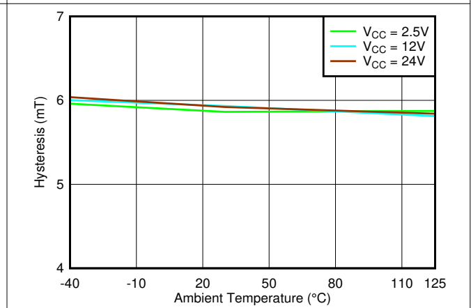
Figure 7-44. Hysteresis_Z vs. Temperature
