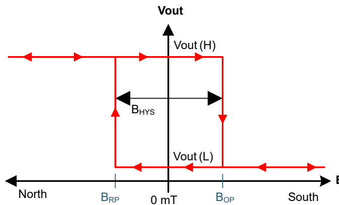
Figure 8-2. Latch Functionality
