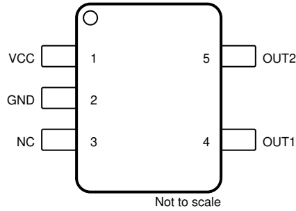
Figure 6-1. DBV Package 5-Pin SOT-23 Top View
