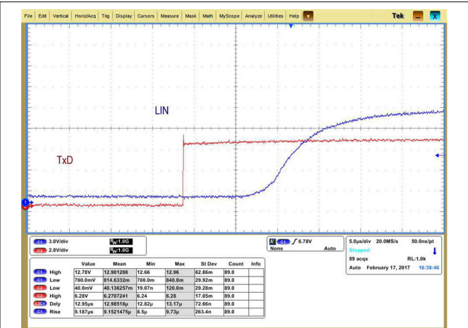
Figure 9-3. Dominant to Recessive Propagation
