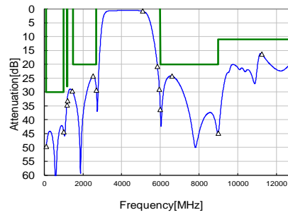
High band-Port S31
