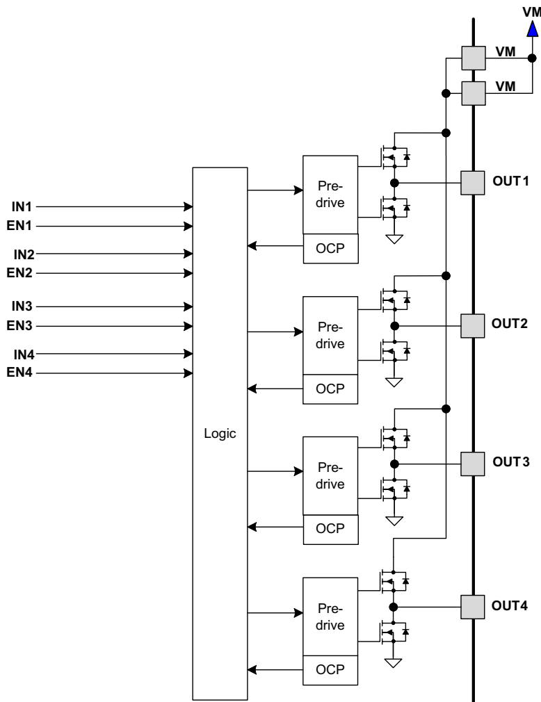
Figure 5. Motor Control Circuitry
