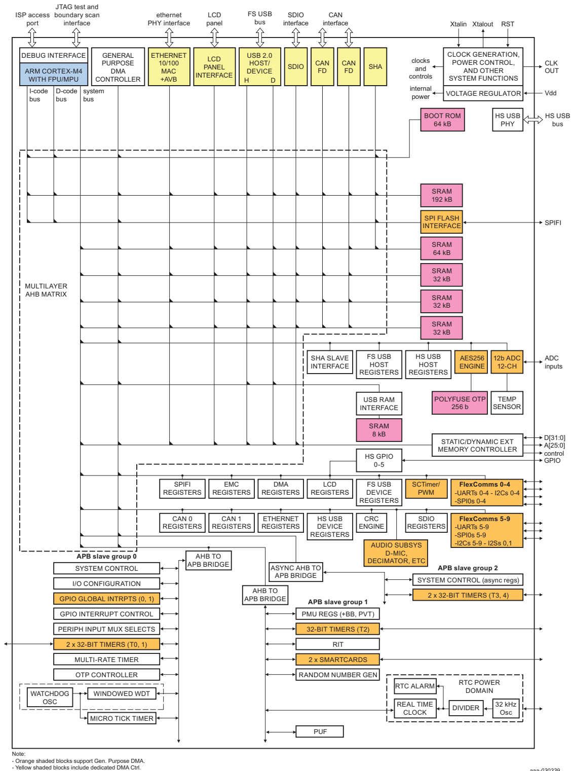
Fig 4. LPC540xx/LPC54S0xx Block diagram
