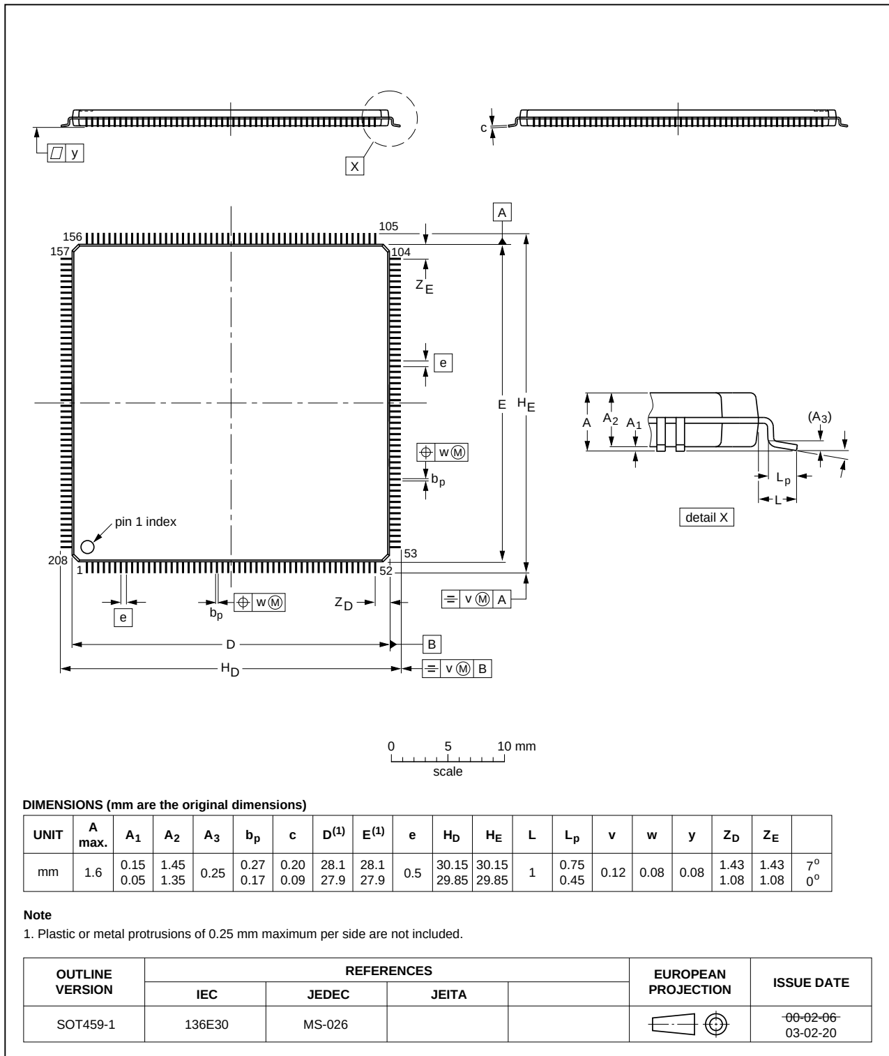
Fig 51. LQFP208 package
