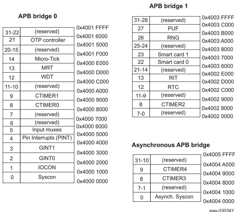
Fig 10. LPC540xx/LPC54S0xx APB Memory map
