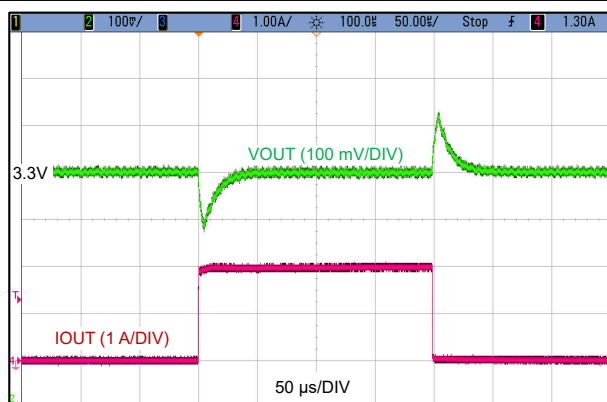
Figure 9-4. Load Transient, 0 A to 2 A, 1 A/ \mu\text{s}
