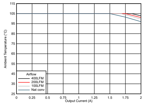
The device is soldered to a 64-mm \times 83-mm, 4-layer PCB. Figure 7-20. Safe Operating Area ( V_{OUT} = 3.3\text{ V} )
