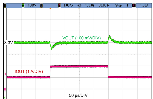
Figure 9-5. Load Transient, 1 A to 2 A, 1 A/ \mu\text{s}
