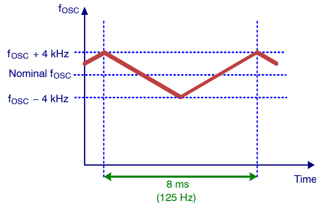
Figure 57. Frequency Modulation of the Maximum Switching Frequency
