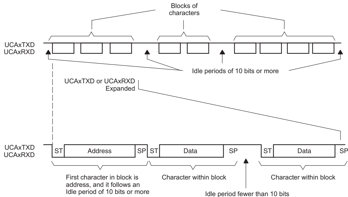
Figure 39-3. Idle-Line Format
