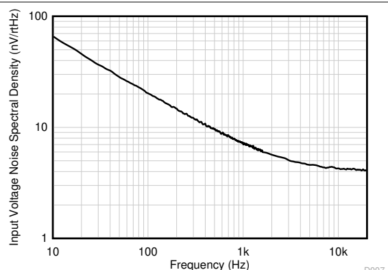
Figure 5-26. Input Voltage Noise Spectral Density vs Frequency
