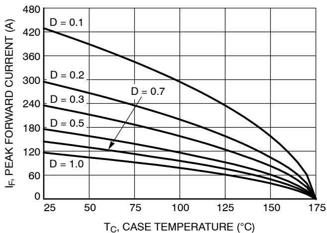
Figure 3. Current Derating
