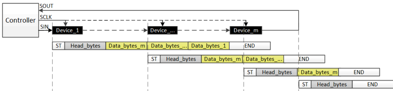
Figure 7-23. Data Write Command with Non-Broadcast
