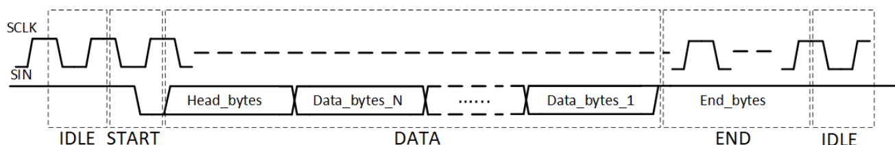
Figure 7-17. CCSI Frame
