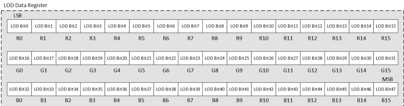
Figure 7-9. Bit Arrangement in LOD Data Register
