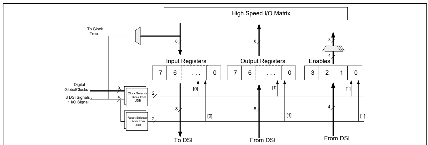
Figure 7 Port Interface
