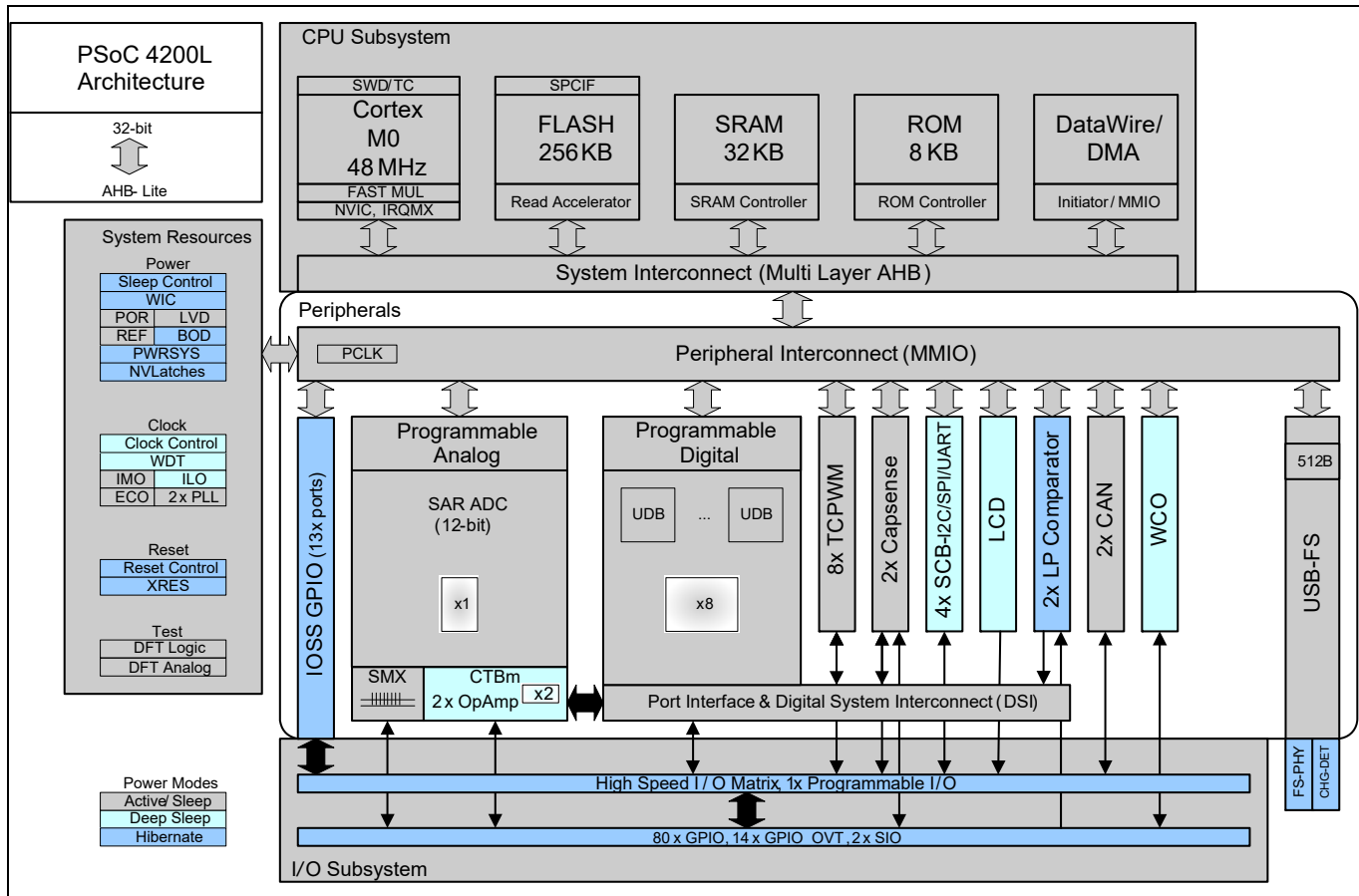
Figure 2 Block diagram
