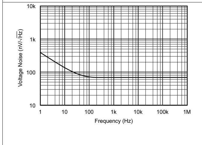
Figure 9. Output Voltage Noise Spectral Density vs Frequency
