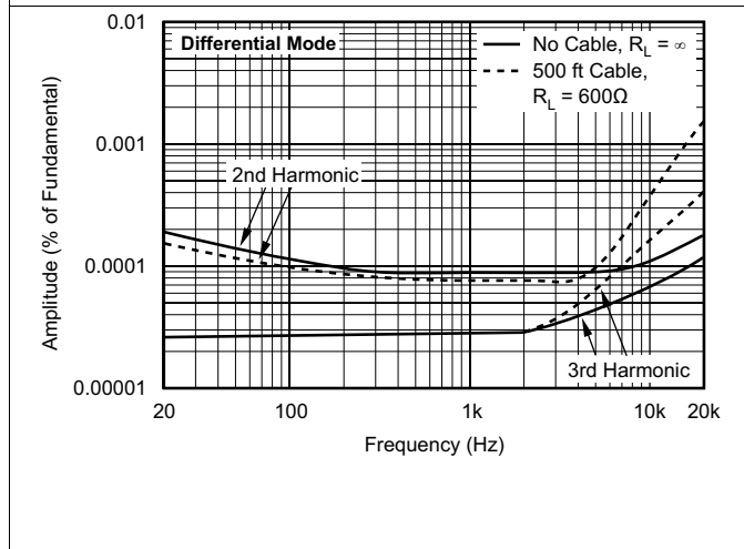
Figure 7. Harmonic Distortion Products vs Frequency
