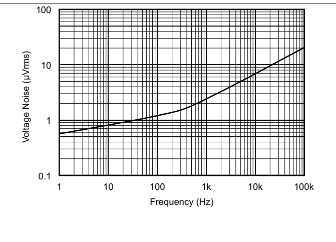
Figure 10. Output Voltage Noise vs Noise Bandwidth
