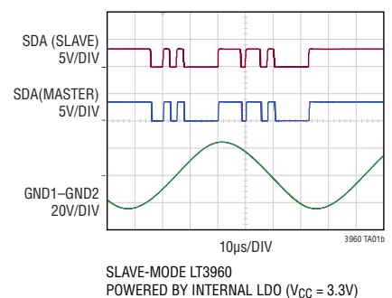
Receiving I 2 C Traffic Across \pm 25V Common-Mode Differential
