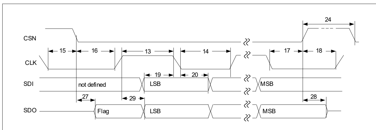
Figure 80 SPI Timing Diagram
