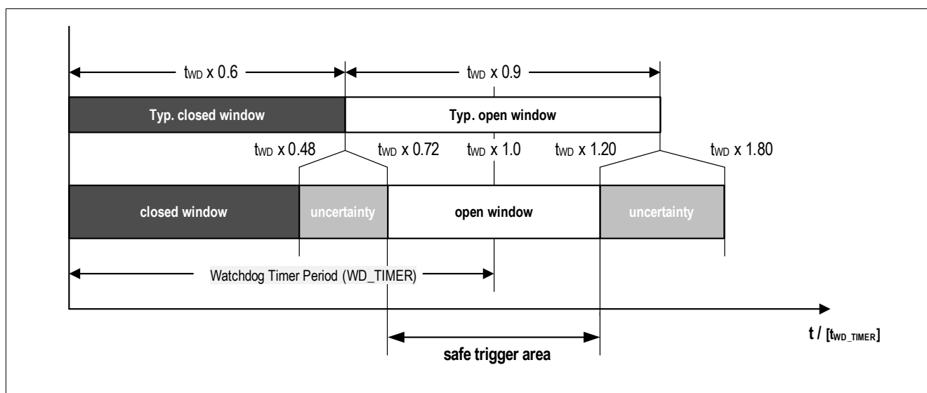
Figure 67 Window Watchdog Definitions
