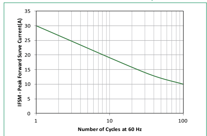
Figure 8 - Maximum Non-Repetitive Forward Surge Current Uni-Directional Only
